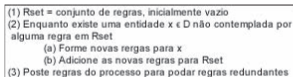
Figure 7. Algoritmo Rule Learning, extraído de Sarawagi (2008)
